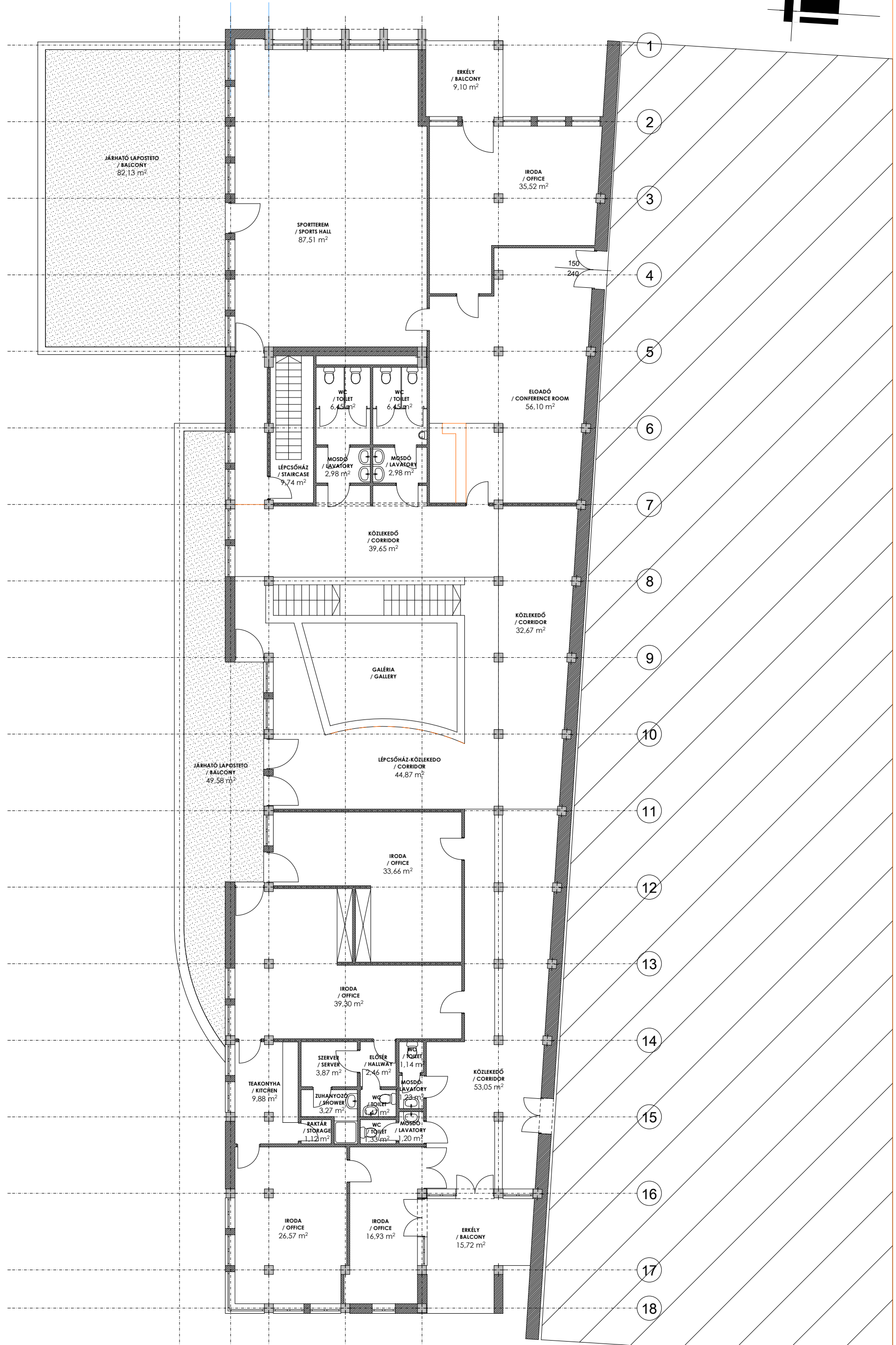
EMELET ALAPRAJZA / WEST WING OF BUILDING FLOOR
